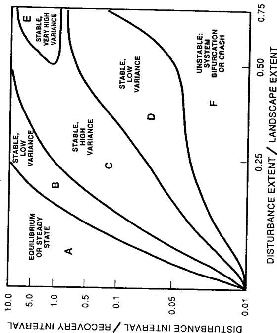
FIGURE 11.6 Landscape disturbance state space. Adapted from Turner et al. (1993).
